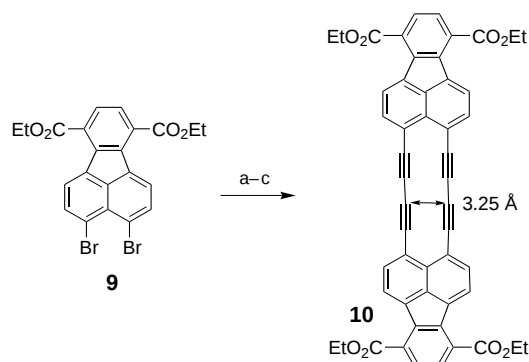
Scheme 2. Synthesis of 10 . Reagents and conditions: a) \text{Me}_3\text{SiCCSnBu}_3/[(\text{Ph}_3\text{P})_2\text{PdCl}_2] ; b) \text{K}_2\text{CO}_3 in \text{EtOH/THF} ; c) \text{CuCl/TMEDA} in \text{CH}_2\text{Cl}_2 .
